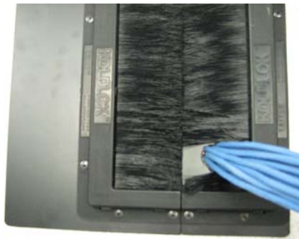
Figure 4. The position of cable bundles in brush-style grommets can move bristles out of position to reduce sealing effectiveness. In addition, bristles can sag, degrade, or break off over time.
