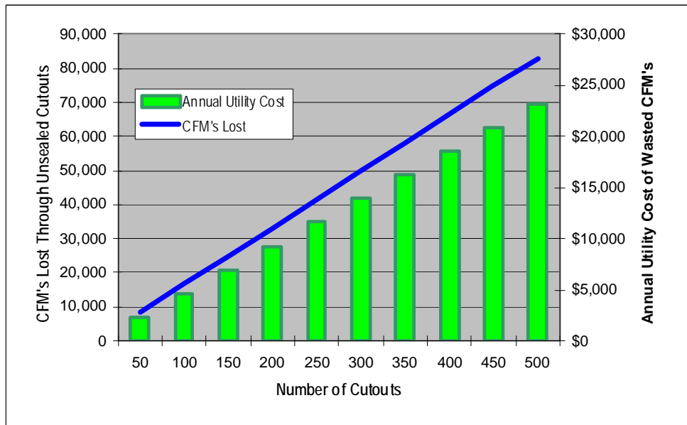
Figure 2. The Cost of Unsealed Cable Cutouts (assumes 4.5 in. x 6.5 in. cutout spaces)
